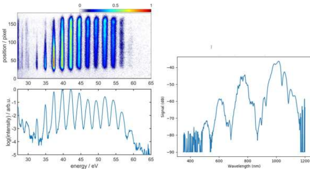
Left-hand side: Extreme ultraviolet spectrum generated by the HR1 laser in Argon. Right-hand side: High-order harmonic radiation generated in ZnSe by th Mid-IR laser
